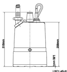
W1: lowest running water level
